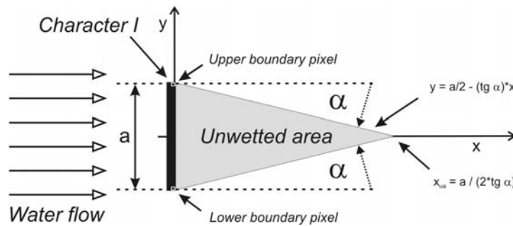
Figure 6: Unwetted area definition
