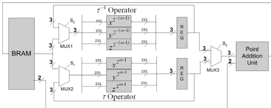
Figure 1: A hardware architecture for scalar multiplication on the NIST Koblitz curve K-233.
