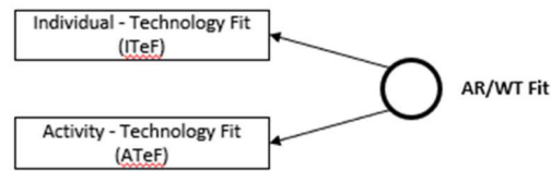
Figure 3: AR/WT Fit construct, adapted from [Parkes 2013]
