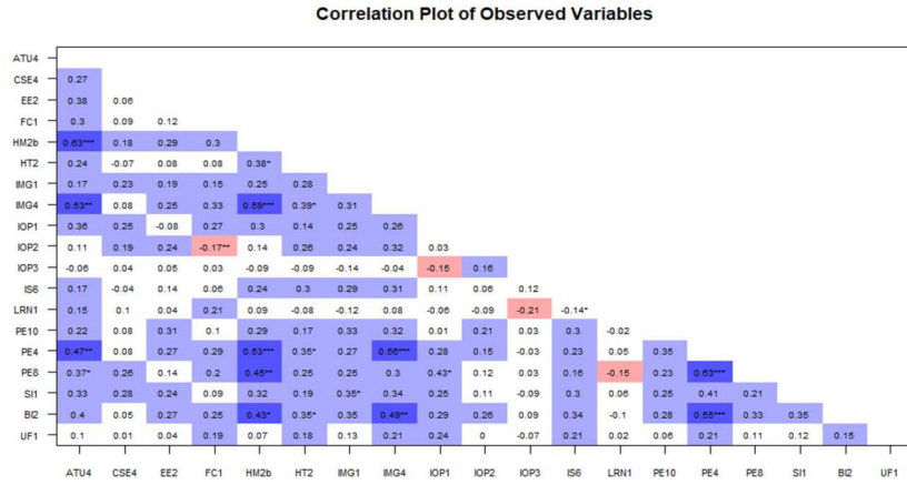
Figure 7: Correlation Plot of Observed Variables
