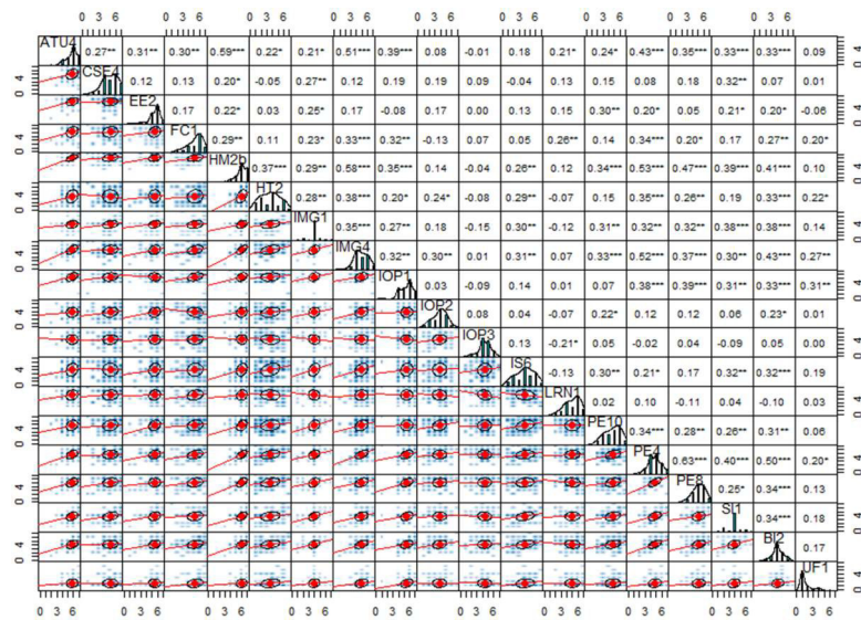
Figure 5: Spearman Rank Correlation of Observed Variables
