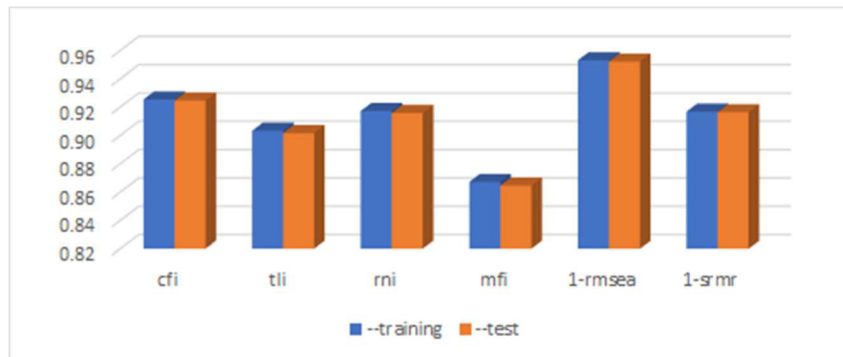
Figure 10: High-fold Cross-validation Results
