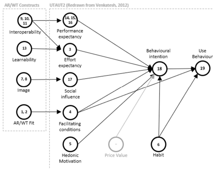
Figure 4: Research Model (showing item allocation)
