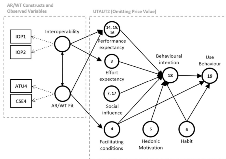
Figure 8: The Final SEM Model
