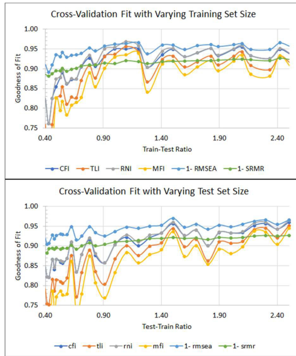
Figure 9: Changes to Fit Indices with Varying Sampling Size
