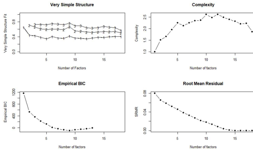
Figure 6: 'Number of Factors' Results
