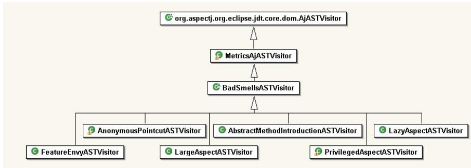
Figure 1: Class hierarchy of the AspectJ extension
