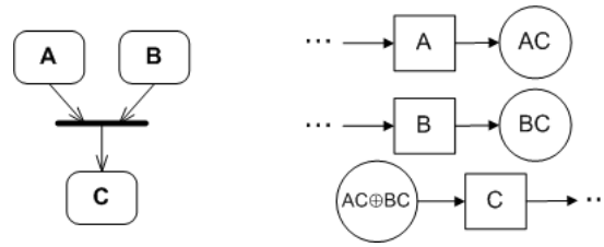
Figure 10: Mapping for join nodes
