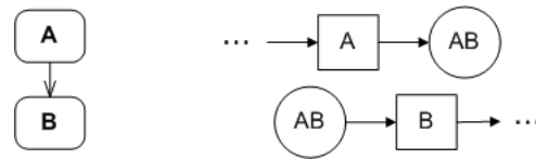
Figure 6: Mapping for sequential composition of action nodes
