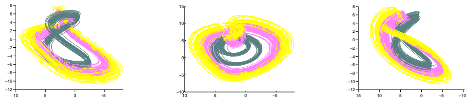
Figure 5: Three different perspectives (front, top and side views) of the curves obtained from the Iris data set when t = s .
