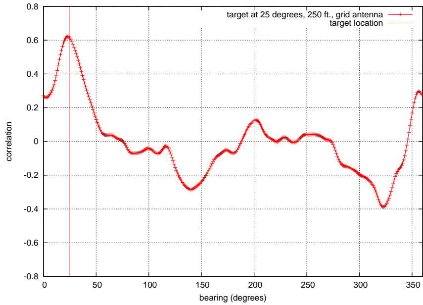
Figure 6: Correlation values of the first June 10 grid antenna trial with the April 11 training data; the maximum correlation occurs at 23°.
