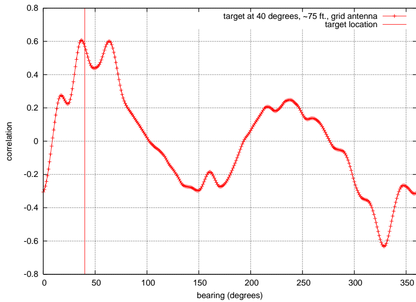
Figure 7: Correlation values of the second June 10 grid antenna trial with the April 11 training data; the maximum correlation occurs at 37°.
