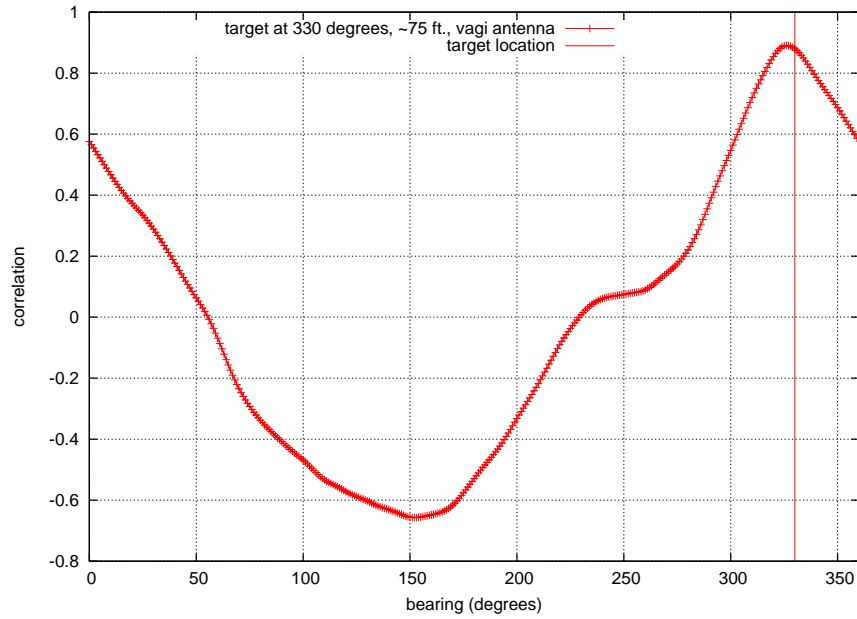
Figure 8: Correlation values of the June 16 Vagi antenna trials, with the first trial as training data and the second as testing; the maximum correlation occurs at 326^\circ .
