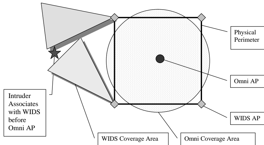
Figure 1: WIDS access point protecting a perimeter
