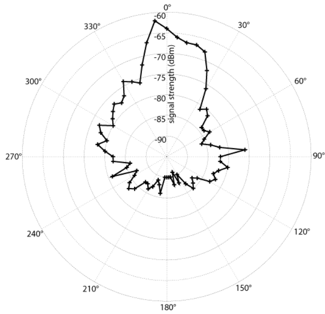
Figure 3: Vagi signal strength versus angle, June 16 2003. Target is at 0 degrees bearing (up), approximately 150 feet from the antenna.
